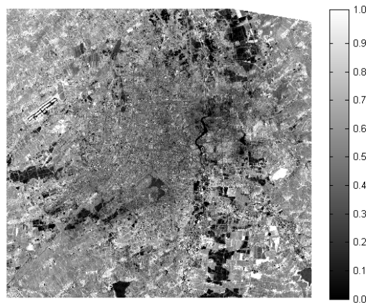
Figure.4d Fraction image of soil in 1993
