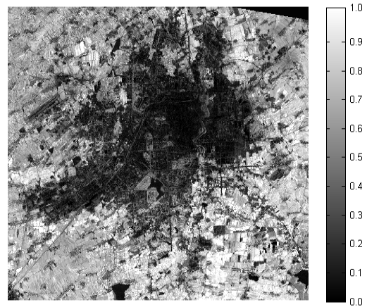
Figure.4c Fraction image of vegetation in 1993
