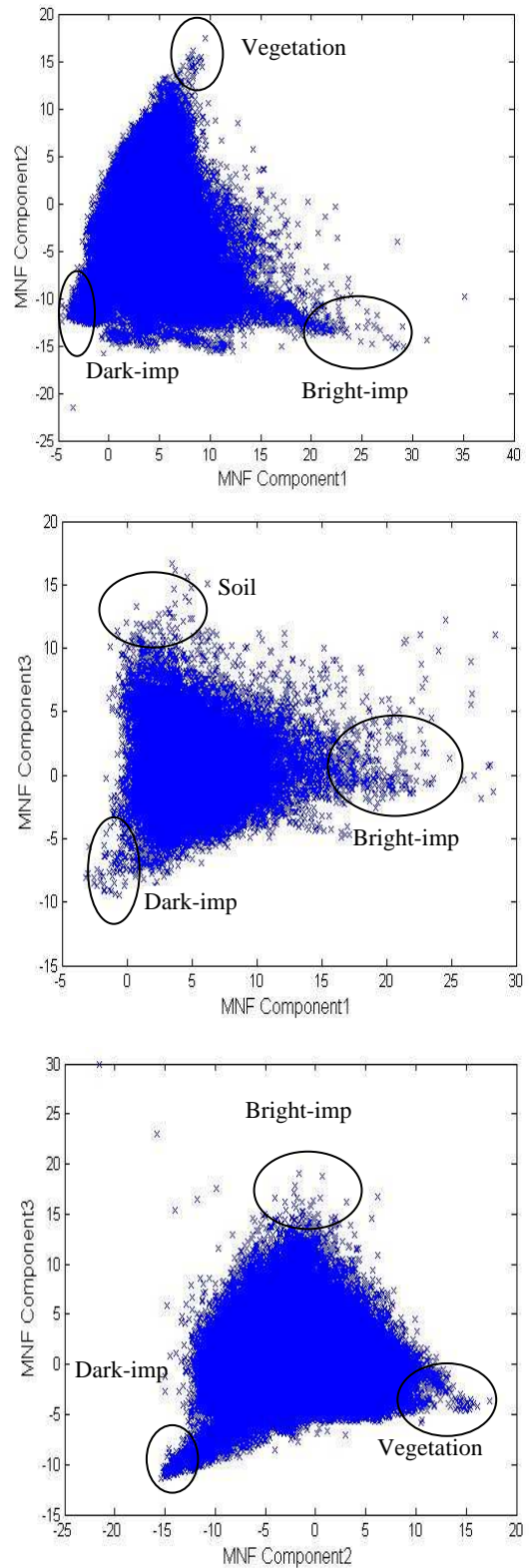
Figure.3 Feature space represents the first three MNF components. The extreme pixel clusters which bound almost all other pixels in these three feature spaces were delineated as endmembers. High albedo (e.g. concrete, clouds, and sand), low albedo (e.g. water, shade and asphalt), vegetation (e.g. crop, grass and trees), and soil (e.g. bare soil and quarry), were identified according to these feature spaces and their corresponding features obtained from original reflectance data.
