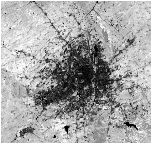
Figure.2a MNF component1
