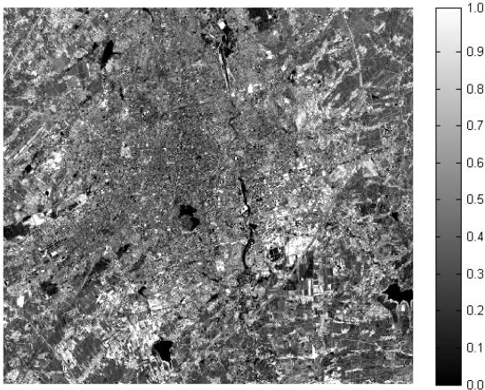
Figure.6d Fraction image of soil in 2003
