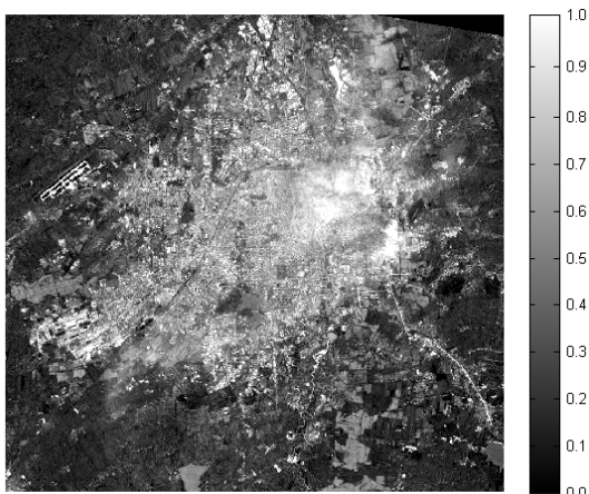
Figure.4a Fraction image of high albedo in 1993
