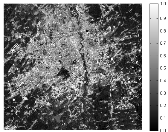
Figure.6a Fraction image of high albedo in 2003
