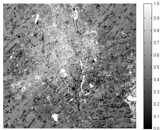
Figure.6b Fraction image of low albedo in 2003
