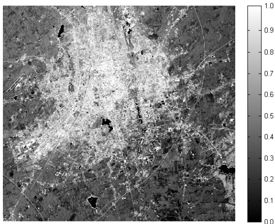
Figure.8b Impervious surface in 2003
