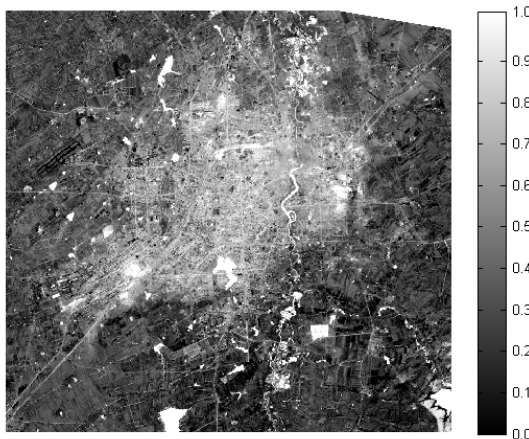
Figure.4b Fraction image of low albedo in 1993
