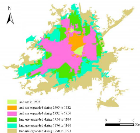
Figure.1 The expansion of Changchun urban area from 1905 to 1993
