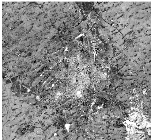
Figure.2b MNF component2
