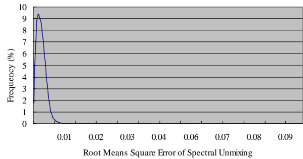
Figure.7 Distribution of Unmixing RMSE
