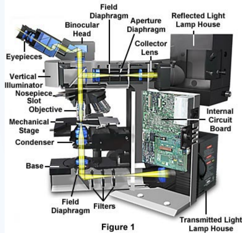
Reflected/Transmitted Light Microscope Configuration
