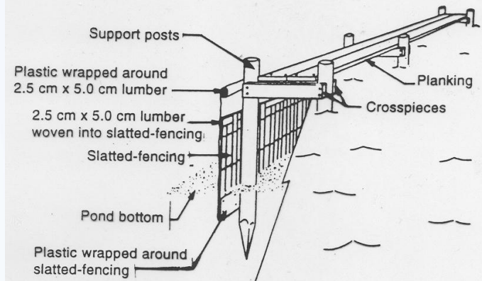
Figure 11. Schematic diagram of a littoral enclosure (Reprinted with permission from Environmental Toxicology and Chemistry 8(12): 1209–1216, Brazner, J. C., Heinis, L. J., Jensen, D. A. A littoral enclosure for replicated field experiments, Copyright 1989 SETAC.)
