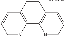
phen 1,10-fenantrolin
