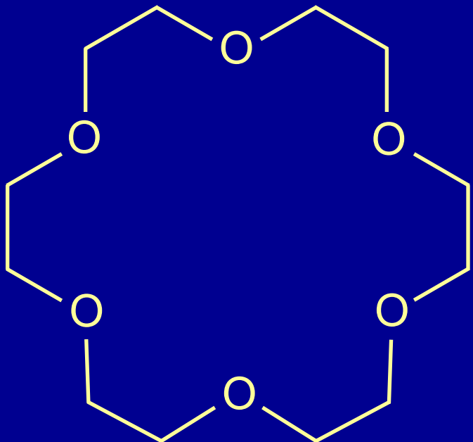
18-crown-6
