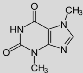
Theobromine (3,7-dimethylxanthine)
