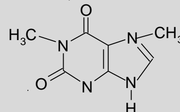
Paraxanthine (1,7-dimethylxanthine)
