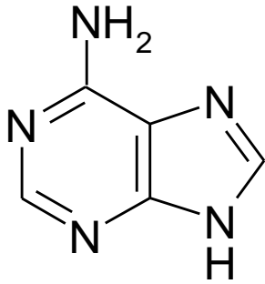
6-amino-purine
