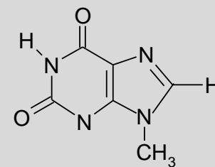
9-methylxanthine
