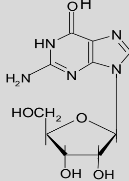
guanosine
