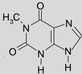
1-methylxanthine
