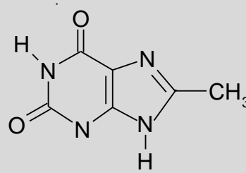
8-methylxanthine
