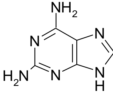
2,6- diamino-purine
