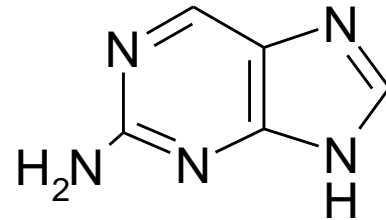
2-amino-purine
