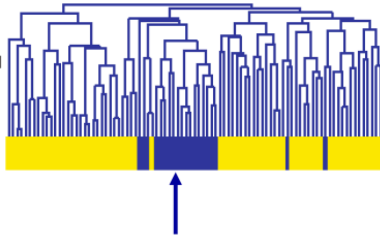
miRNA
