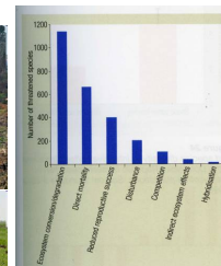
Figure 21 Most threats impact threatened bird species through ecosystem conversion and degradation, but many cause direct mortality also.
