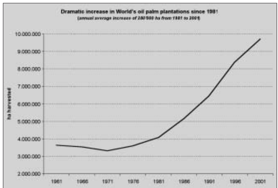
Fig. 2: Growth in global oil palm plantations, 1961 – 2001
