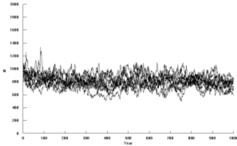
Figure 5.8. Trajectories of 10 simulated populations with initial size of 1000 and the worst mortality rates
