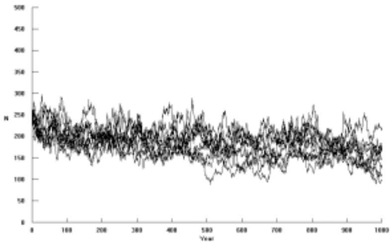
Figure 5.9. Trajectories of 10 simulated populations with initial size of 250 and the worst mortality rates
