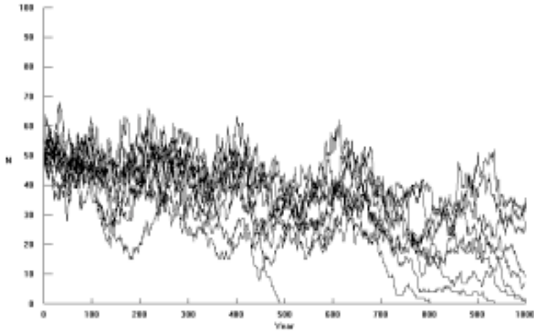
Figure 5.4. Trajectories of 10 simulated populations with initial size of 50 and the best mortality rates
