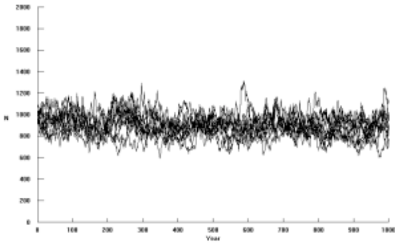
Figure 5.5. Trajectories of 10 simulated populations with initial size of 1000 and medium mortality
