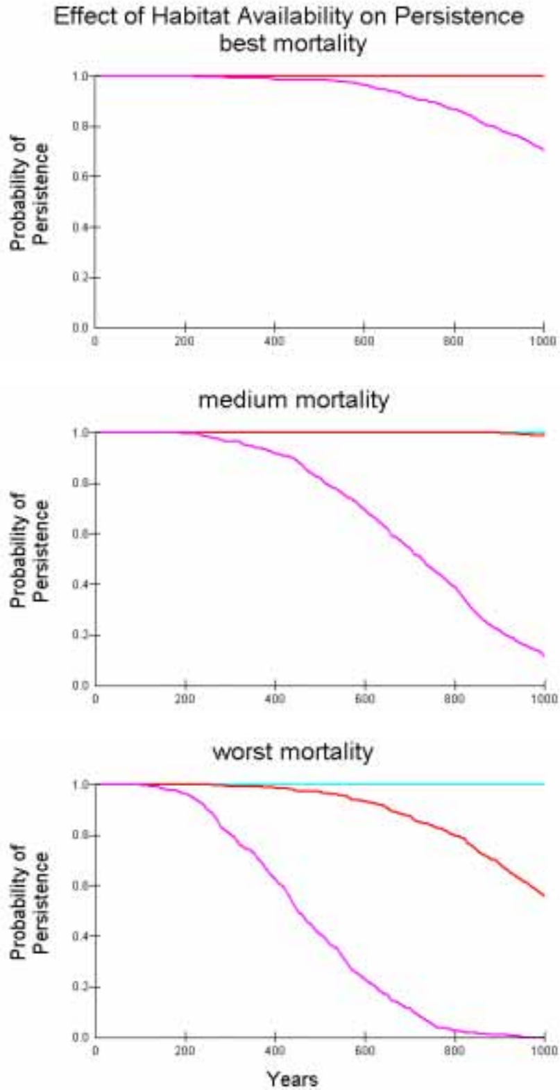
Figure 5.11. Probability of persistence for populations of maximum and initial size of 1000, 500, 250, 100, and 50 (top to bottom, with some top lines superimposed), subjected to three levels of natural mortality
