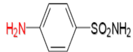
Sulfanilamid antibiotikum
