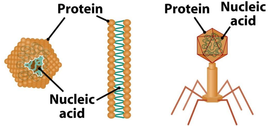
Icosahedral
