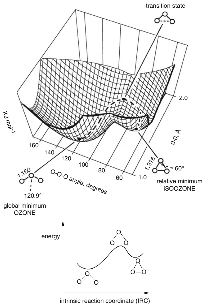
Fig. 2.7 The ozone/isozone potential energy surface (calculated by the AM1 method; Chapter 6 ), a 2D surface in a 3D diagram. The dashed line on the surface is the reaction coordinate (intrinsic reaction coordinate, IRC). A slice through the reaction coordinate gives a 1D “surface” in a 2D diagram. The diagram is not meant to be quantitatively accurate
