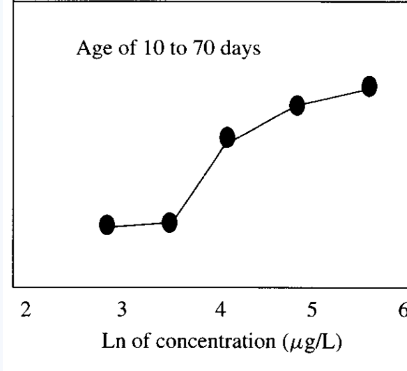
Fig. 6.1. Density-dependent, natural mortality can obscure the concentration–effect relationship for caddisfly larvae exposed to 4,5,6-trichloroguaiacol. There was no discernible relationship for larvae \leq 9 days old, an age class with high levels of natural, density-dependent death. Note the high mortality in all treatments. (Probit values of 4 and 5 correspond to 16 and 50% mortality, respectively.) There was a clear relationship between mortality and toxicant concentration of older larvae ( >9 to 70 days old). (Modified from Figure 4A&B of Petersen and Petersen 1988)
