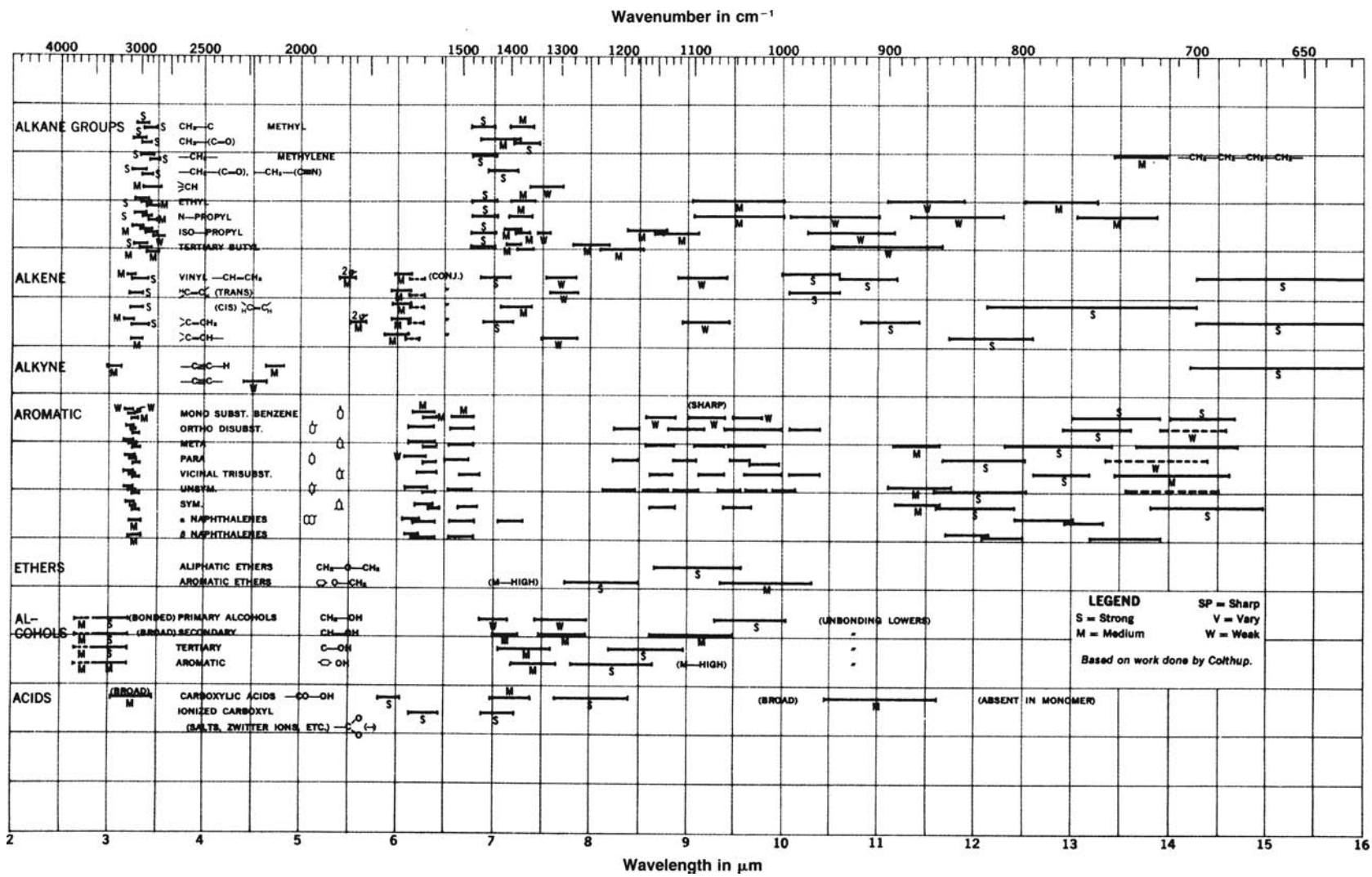
INFRARED CORRELATION CHARTS
