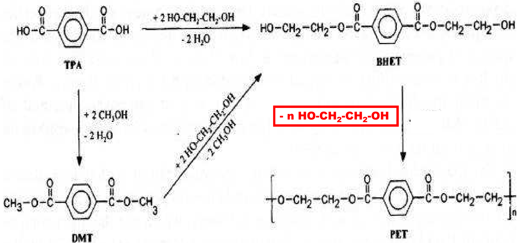
Scheme 2.1 Routes of PET preparation.
