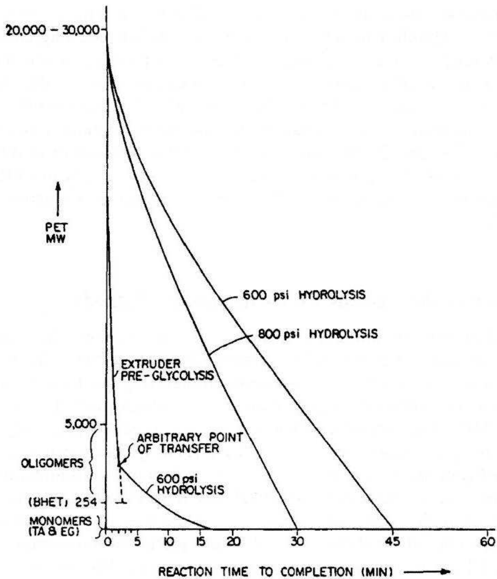
Figure 2.5 Change of the PET molecular weight along the time for different degradation treatments. 70
