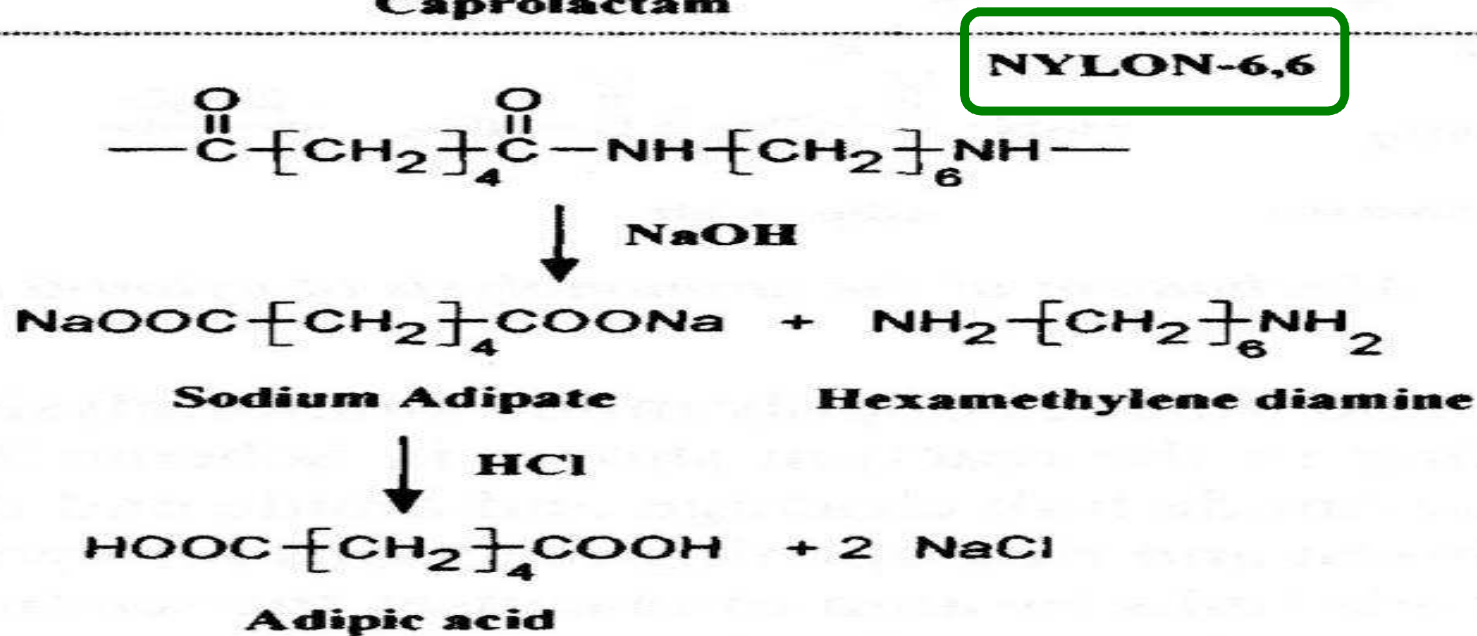
Scheme 2.8 Hydrolysis of nylon-6 and nylon-6,6. 2
