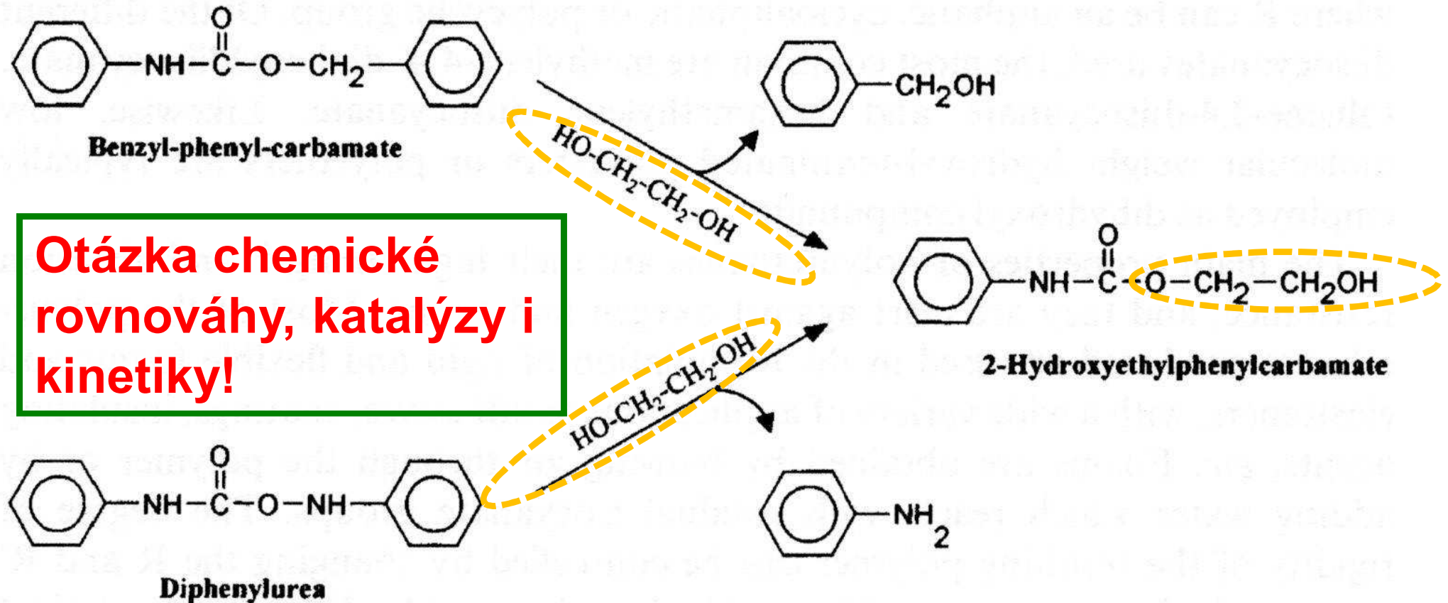
Scheme 2.3 Glycolysis of benzyl-phenyl-carbamate and diphenylurea. 82
