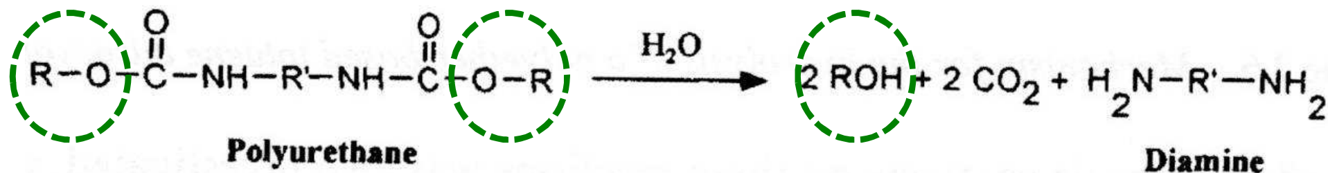
Scheme 2.4 Polyurethane hydrolysis .
