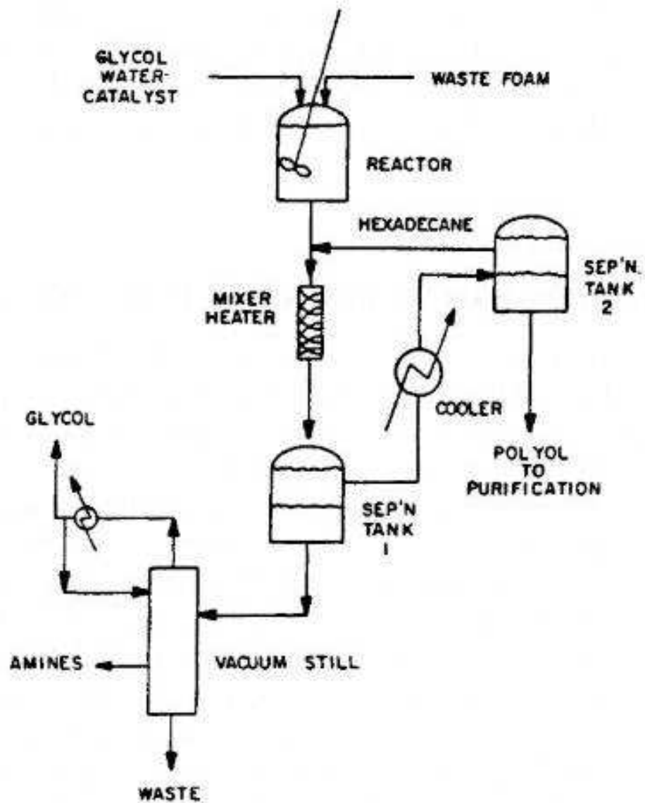
Figure 2.7 Flow diagram of the Ford hydroglycolysis process for the degradation of polyurethanes. 94
