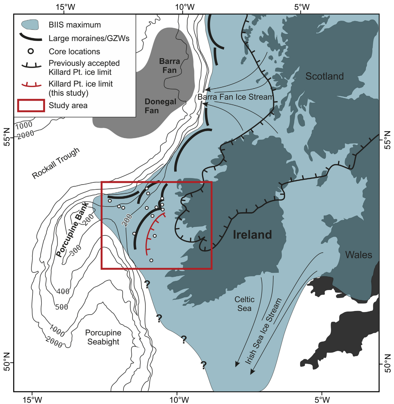
Fig. 1. Regional map locating the study area (shown in Fig. 2) and core locations amongst prominent glacial landforms, ice streams and the last BIS's maximum extent (Sejrup et al., 2005; Scourse et al., 2009; Clark et al., 2012a; Peters et al., 2015). The 'Previously accepted Killard Point ice limit' is compiled from reconstructions by McCabe et al. (1998) in Ireland and the theoretical model of BIS extent at approximately the 17 ka BP isochrone synthesised by Clark et al. (2012a).
