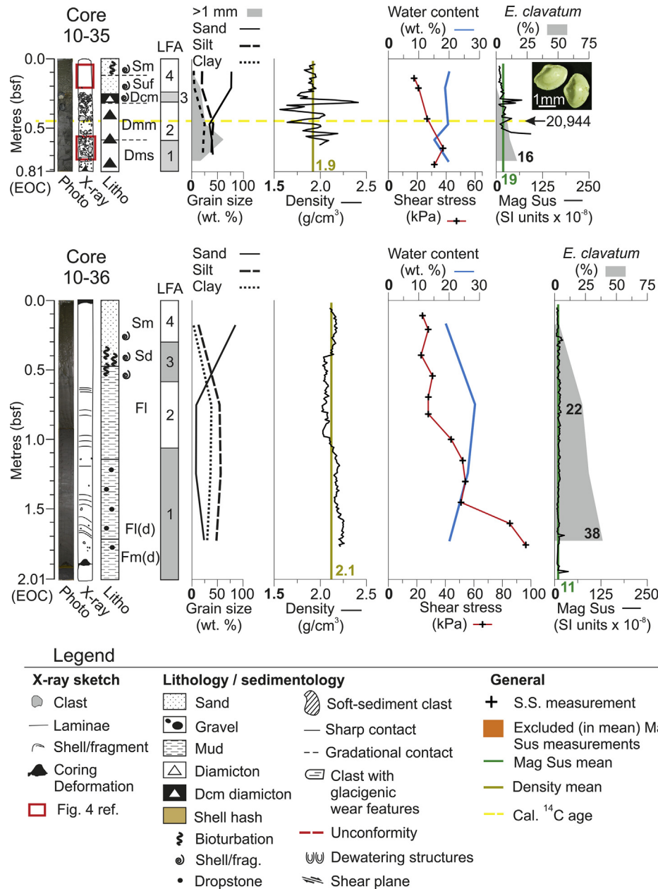
Fig. 5. Plots of core data from the western Irish continental shelf. From left: true-colour photograph, sketch of prominent structures discerned by x-radiograph analyses, log of lithology and sedimentary structures, lithofacies abbreviations and extents of LFAs, grain size data, sediment density (wet bulk) and (in cores 10-40 and 14-59) counts of lithic fragments >1 mm, sediment shear strength and water content (percent by weight), magnetic susceptibility and relative abundance of the benthic foraminifer Elphidium excavatum forma clavatum . AMS radiocarbon sample locations (m bsf) are marked by horizontal, dashed yellow lines; ages are provided in Cal BP and photographs of the dated materials are shown. (For interpretation of the references to colour in this figure legend, the reader is referred to the web version of this article.)
