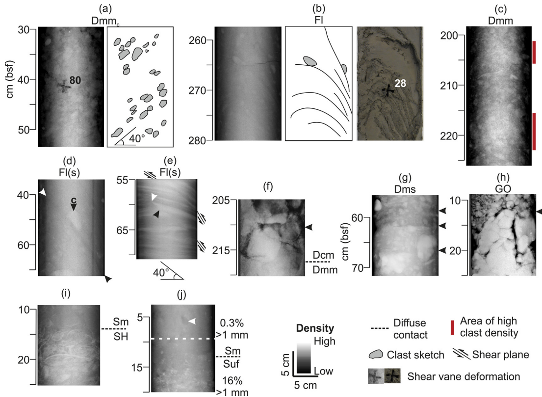
Fig. 4. Representative x-radiograph facies. (a) X-radiograph and structure sketch of in Dmm c from core 10-38 exposing a ~40° preferential clast alignment and showing the location of a shear stress measurement of 80 kPa. (b) X-radiograph, structure sketch and photograph of deformed FI from core 14-59 revealing apparent clast alignment to strain and showing the location of a shear stress measurement of 28 kPa. (c) Dmm from core 10-40 exposing rhythmic areas of high clast concentration. (d) Clast-rich FI(s) from core 14-57 exposing a prominent shear plane (top = white arrow, bottom = black arrow) with a large (~3-cm long) clast (arrow labelled 'c') aligned in the direction of shear. (e) FI(s) from core 14-41; well-defined laminae reveal a ~40° reverse fault with an offset of ~2 cm (top of offset = white arrow, bottom of offset = black arrow). (f) Dcm with a diffuse lower contact overlying Dmm in core 14-59; black arrow marks an area devoid of large clasts but filled with interstitial sandy matrix. (g) Dms from core 10-35 exposing clast-rich, horizontal stratification; black arrows mark contacts between select strata. (h) GO from core 10-38; black arrow marks an area of void space between clasts. (i) Diffuse contact between Sm and underlying SH in core 14-54; large shells are exposed as light-grey curvilinear shapes. (j) Diffuse contact between Sm and underlying Suf in core 10-35; white dashed line marks the location of the GSA analyses that yielded 0.3% > 1 mm lithic fragments; GSA analysis that yielded 16% > 1 mm lithic fragments was taken at the bottom of the core section shown; white arrow marks an area of relatively low-density, poorly-sorted, shell-fragment-rich material interpreted as an infilled burrow (bioturbation); shell fragments are exposed as light-grey/white.
