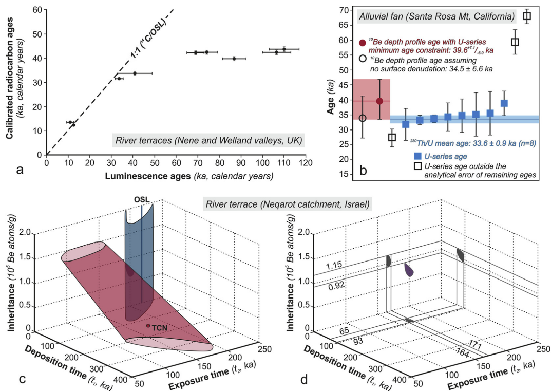
Fig. 9. a) Comparison of ^{14}\text{C} (uncertainties: one standard deviation) and OSL (uncertainties: one standard error) dates from the same fluvial sequences. Calibration of radiocarbon dates: (Reimer et al., 2004) for ages <26 ^{14}\text{C} ka BP and Fairbanks et al. (2005) for ages >26 ^{14}\text{C} ka BP. Note the systematic age underestimation of ^{14}\text{C} dating beyond the 29–35 ka limit. After Briant and Bateman (2009); b) Plot showing ^{10}\text{Be} depth profile ages and ^{230}\text{Th}/\text{U} ages for alluvial fan deposits, both with 2\sigma error. Shaded red and blue boxes represent the mean ^{10}\text{Be} exposure age and mean U-series age, respectively. Note the slightly younger age range of ^{230}\text{Th}/\text{U} dating (minimum age) than the one defined by the depth profile, proving the usefulness of this combined approach. After Blisniuk et al. (2012); c, d) Integrated ^{10}\text{Be} depth profile and OSL model results in the model parameter space of deposition time ( t_1 ), exposure time ( t_2 ), and ^{10}\text{Be} inheritance for a single alluvial sequence. The cosmogenic nuclide model best fit (thick red dot) with the 68% confidence level envelope around it (red surface), the OSL model best fit (vertical blue line) with the 68% confidence level envelope around it (blue surface) and the intersection of the two confidence surfaces (dark surface) are shown on (c). The intersection alone is represented on (d), with its 2D projection onto the axial planes (grey surfaces) and further 1D reprojection onto the axes (grey labelled lines). After Guralnik et al. (2011). (For interpretation of the references to colour in this figure legend, the reader is referred to the web version of this article.)
