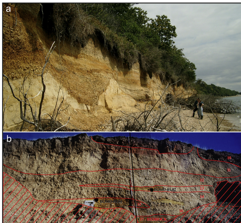
Fig. 4. a) A good sampling location for Luminescence dating at Stanswood Bay, Hampshire, England (Briant et al., 2006). The thickest sand bed at the base is Mesozoic in age, but samples were taken from thick sand beds above the gravel channel (as shown and above the photo out of view); b) Less optimal sampling location for Luminescence dating at Barton on Sea, Hampshire, England (Briant et al., 2006). Field gamma spectrometry was undertaken to mitigate the complex dose rate effect of the thinner sand lenses.
