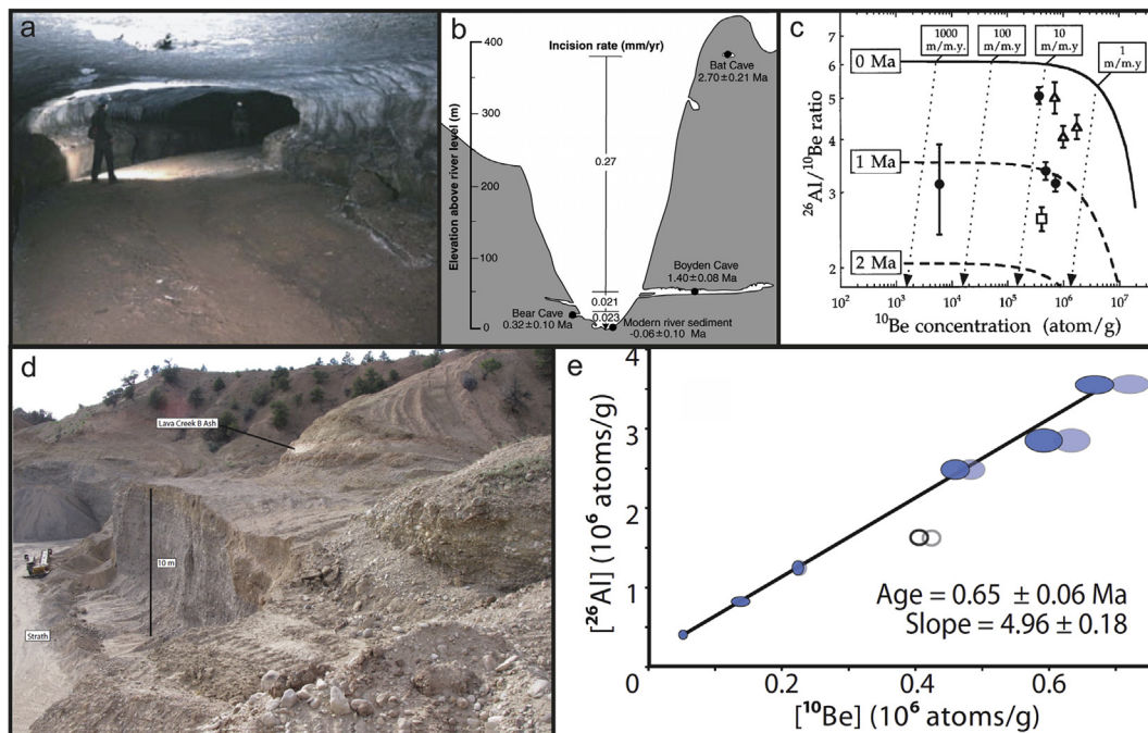
Fig. 8. Burial dating: application of two sampling strategies to different fluvial archives (left), exemplified by dating results (right). a) Horizontal, abandoned phreatic tube, partly filled with river sediments (Cumberland river catchment, Appalachian mountains, USA). Note the regular elliptical cross-section of the former phreatic passage. After Anthony and Granger (2007), photo: D. Granger; b) Topographic cross-section across the South Fork river canyon (Sierra Nevada, USA) displaying the multi-level cave system in which burial dating was performed. Note the significant decrease of incision rates toward present. After Stock et al. (2004); c) erosion-burial diagram, the bold line represents the ^{26}\text{Al}/^{10}\text{Be} ratio in steadily eroding rocks whereas the dashed curves refer to equal burial duration (dotted lines refer to pre-burial erosion rates). All samples plot beneath the bold line and have therefore experienced burial (New river, Appalachian mountains, USA). After Granger et al. (1997); d) \sim 10 m-thick, gravel terrace body overlain by a tephra layer, sampled at the base for isochron burial dating because of insufficient shielding to cosmic rays (Gunnison river, Colorado plateau, USA). After Darling et al. (2012), photo: L. Crossey; e) Graphical representation of burial dating isochron for a gravel terrace, the burial age is calculated from the slope of the regression line (Sundays river, South Africa). After Erlanger et al. (2012).
