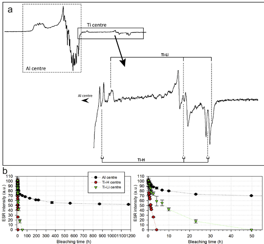
Fig. 6. a) Examples of ESR spectra of Al and Ti centres measured in quartz. Modified from Duval and Guilarte (2015); b) Decay of the ESR intensity of the different centres Al, Ti-Li and Ti-H under UV exposure. This laboratory bleaching experiment was performed with a SOL2 sunlight simulator (Dr Hönle) on a quartz sample from the Morée-Villeprovert locality, France.
