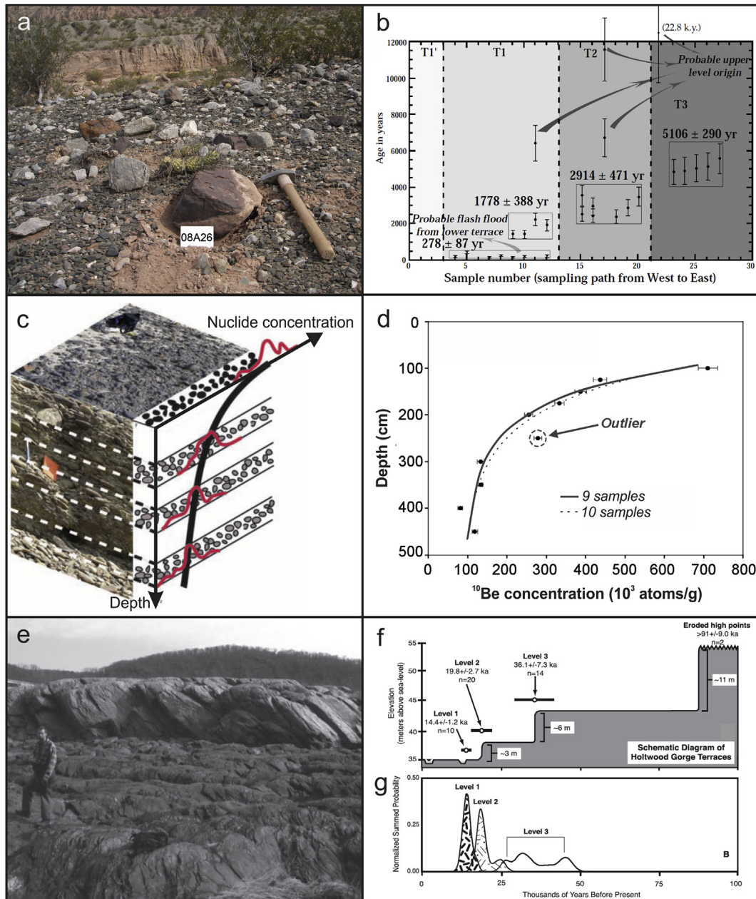
Fig. 7. Surface exposure dating: application of distinct sampling strategies to different fluvial archives or landforms (left), exemplified by dating results (right). a) Sandstone boulder lying at the surface of an alluvial fan, sampled for ^{10}\text{Be} concentration measurement (Escondida creek, Andean Precordillera, Argentina). After Schmidt et al. (2011); b) Mean surface exposure ages (bold numbers), calculated from ^{10}\text{Be} and ^{26}\text{Al} concentration measurements in individual clasts samples, for three fan terraces displaced by Holocene strike-slip faulting activity (NE Tibet). The young age cluster on T1 is attributed to the occurrence of a recent flash flood (light arrow) whereas the four samples from T1, T2 and T3 with much older apparent ages (dark arrows) are supposed to have been reworked from older deposits but may also have a higher inherited content. Modified after Van der Woerd et al. (1998); c) Sketch of TCN concentrations along a depth profile (bold black curve) in an alluvial sequence deposited in a single event, highlighting a concentration decrease with depth. Red curves represent supposed frequency distribution of nuclide concentrations of individual clasts, illustrating the need to amalgamate tens of clasts. Modified after Ivy-Ochs and Kober (2008); d) measured ^{10}\text{Be} concentrations with 1\sigma error bars along a \sim 4.5 m-deep profile in terrace sediments (Ourthe river, Ardennes massif, Belgium) and modelled curves based on 10 or 9 samples (bold and dashed curves, respectively). Modified after Rixhon et al. (2011); e) two distinct levels of fluvially-carved strath terraces; both bedrock surfaces were sampled for ^{10}\text{Be} concentration measurements (Susquehanna river, Appalachian mountains, USA). After Reusser et al. (2006); f) Sketch summarizing the Late Pleistocene incision in the Susquehanna river based on ^{10}\text{Be} concentrations of distinct strath terraces (with a minimum age for the upper, strongly eroded surface); g) Normalized cumulative probability curves based on the sample numbers of fig. f for the three lower terrace levels. After Reusser et al. (2006). (For interpretation of the references to colour in this figure legend, the reader is referred to the web version of this article.)
