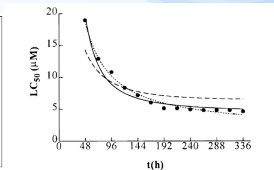
FIGURE 4. Fits of the critical body residues model (CBR, - -), the aqueous critical target occupation model (CTO a , · · ·), and the whole-body critical target occupation model (CTO wb , —) to the LC 50 (t) data of chlordion in the pond snail.
