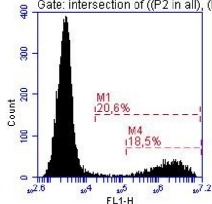
E03 A 3 PEI Gate: intersection of ((P2 in all), (P
