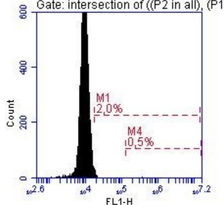
E02 A 2 neon Gate: intersection of ((P2 in all), (P1
