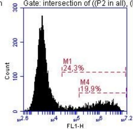
F03 B PEI Gate: intersection of ((P2 in all), (P
