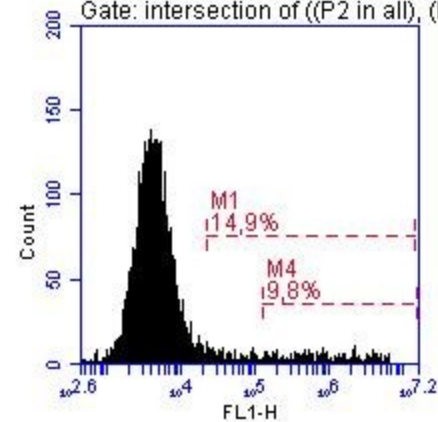
F04 B lipofectamine Gate: intersection of ((P2 in all), (P1 in
