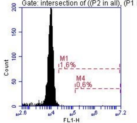
F02 B neon Gate: intersection of ((P2 in all), (P1 in
