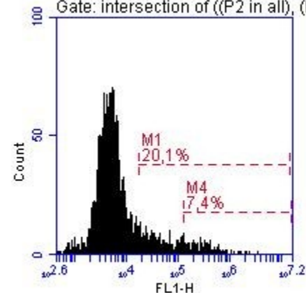
E04 A 4 Lipofectamine Gate: intersection of ((P2 in all), (P1 in
