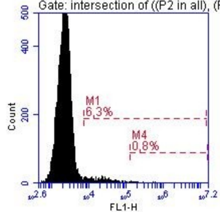
F01 B Fugene Gate: intersection of ((P2 in all), (P
