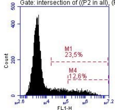
E01 A 1 Fugene Gate: intersection of ((P2 in all), (P1
