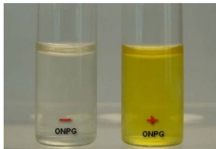
Proteus vulgaris (Left): ONPG Negative Escherichia coli (Right): ONPG Positive
