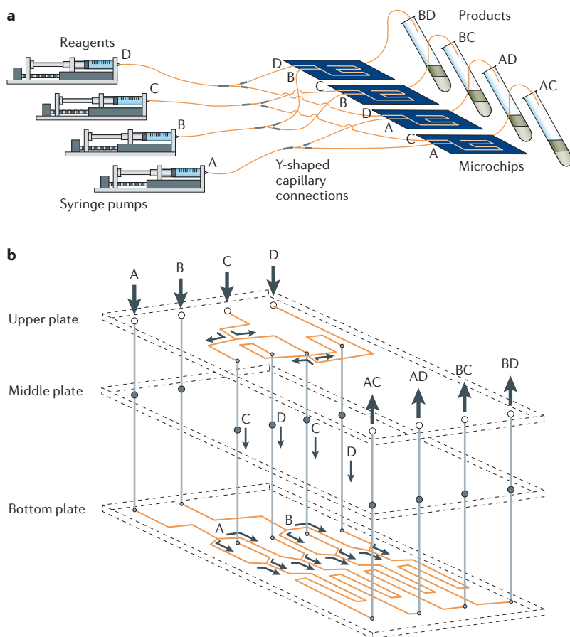
Figure 2 | Combinatorial syntheses in microfluidic chips. a | Schematic views of a microreactor system for 2 × 2 combinatorial syntheses composed of four microchips. b | Schematic views of a microreactor system for 2 × 2 combinatorial syntheses realized in one single three-dimensional microchip 39 .
