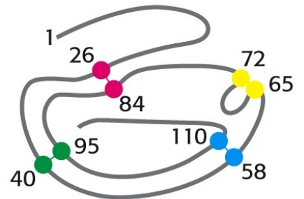
Native ribonuclease
