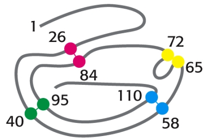
Native ribonuclease
