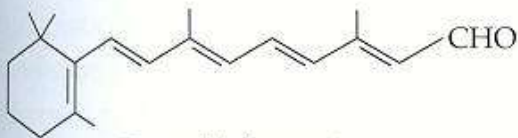
Retinal (all-trans)
