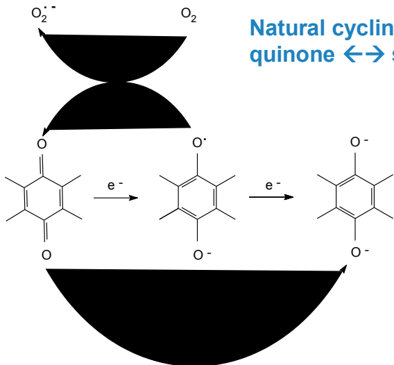
Figure 1. CoQ 10 is an essential component of the electron transport chain within the mitochondria. 2,3
