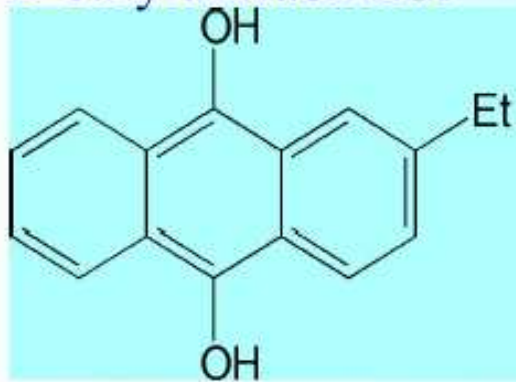
2-ethylantrachinol
