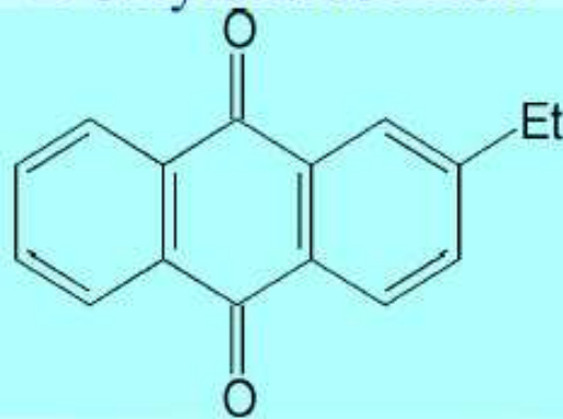
2-ethylantrachinon
