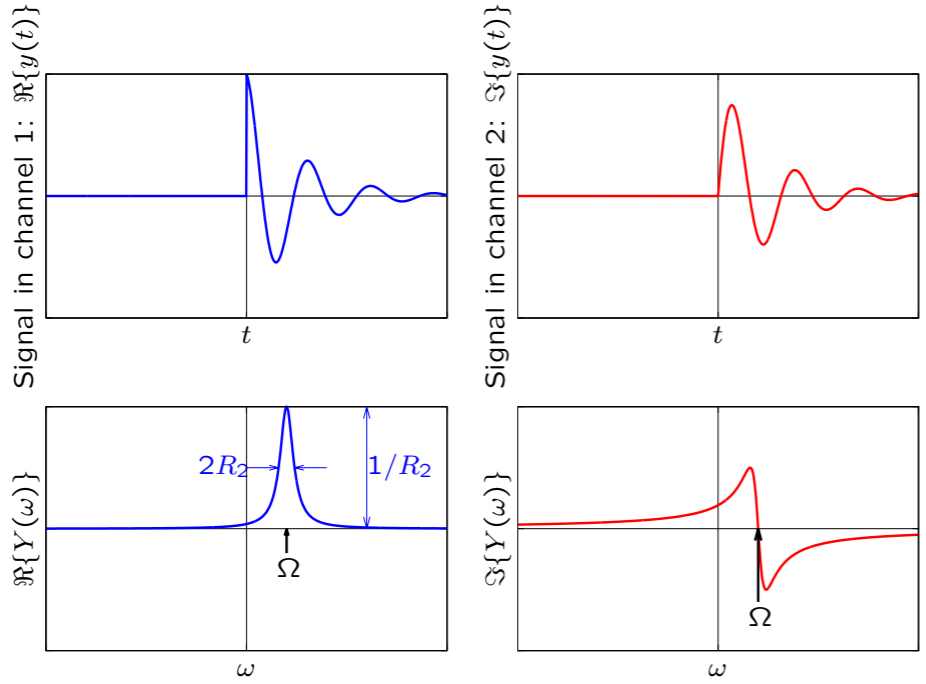
Fourier transformation of ideal signal.
