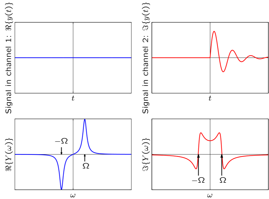
Fourier transformation of sine.
