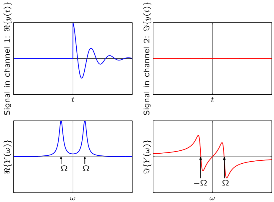
Fourier transformation of cosine.
