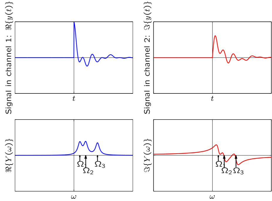
Three Larmor frequencies.
