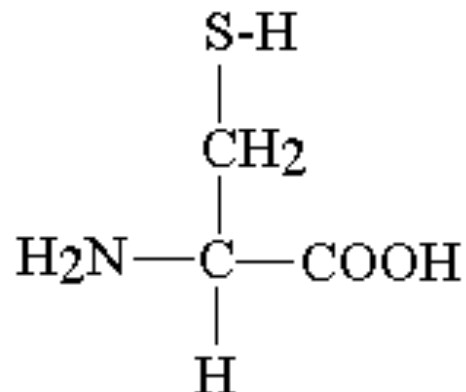
cysteine
