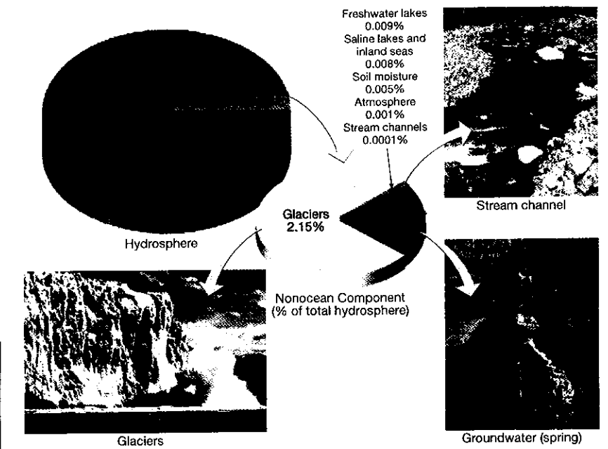
FIGURE 1.14 Distribution of Earth's water. The oceans clearly dominate . When we consider only the nonocean component, ice sheets and glaciers represent nearly 85 percent of Earth's fresh water. Groundwater accounts for just over 14 percent. When only liquid freshwater is considered, the significance of groundwater is obvious . (Glacier photo by Bernhard Edmaier/Photo Researchers, Inc.; stream photo by E. J. Tarbuck; and groundwater photo by Michael Collier)
