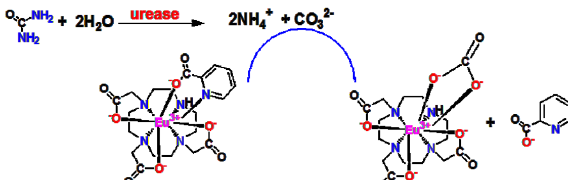
Scheme: The cascade reaction of the ternary [Eu(DO3A)(Pic)]- complex employed for enzymatic determination of urea.
