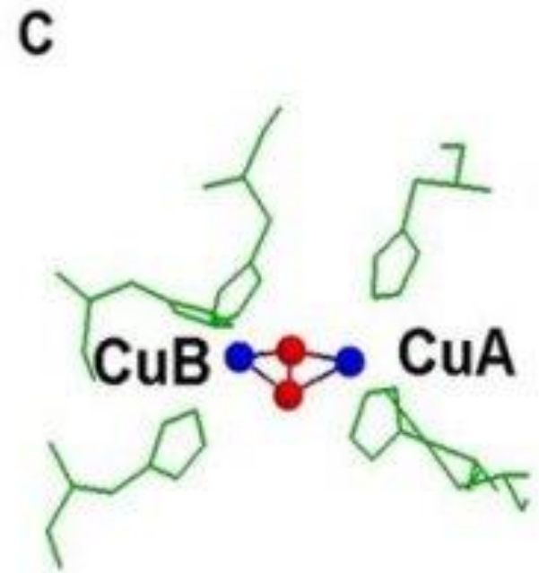
Hemocyanin
