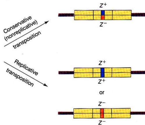
Figure 21-20 Consequences of conservative and replicative transposition. (a) The heteroduplex of homoduplex nature of DNA (see Figure 21-19) is transposed into a target gene. If the starting DNA is heteroduplex, then the resulting DNA will still be heteroduplex only in a conservative, or nonreplicative, pathway. (b) Because the heteroduplex results in a transposed cell that maintains the heteroduplex nature of the DNA during conservative transposition, colonies will arise that are part Z^+ and part Z^- . However, in a replicative pathway, transposition results in individual cells that are either all Z^+ or all Z^- , and all the colonies will either be Z^+ or Z^- .
