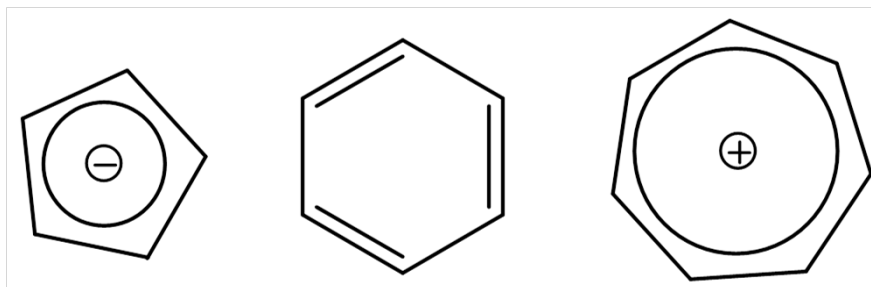
tropylium
