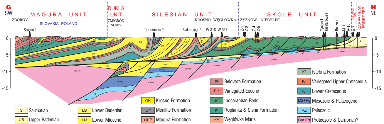
Fig. 6. Integrated geological-geophysical-sections (G–H) Smilno–Rzeszów (after Oszczytko et al., 1998 — supplemented)
