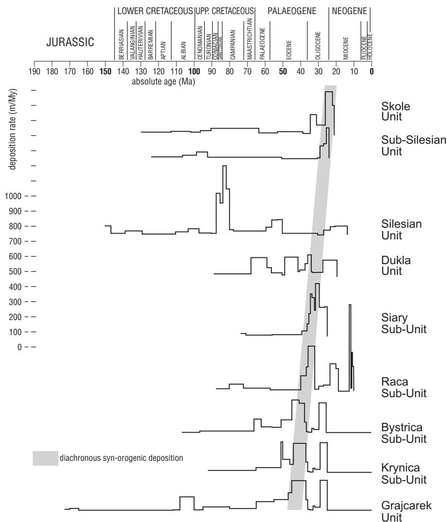
Fig. 9. Diagram of deposition rates versus time for selected synthetic profiles from the Polish Outer Carpathians (after Poprawa et al., 2002b; Oszczytko et al., 2003)
