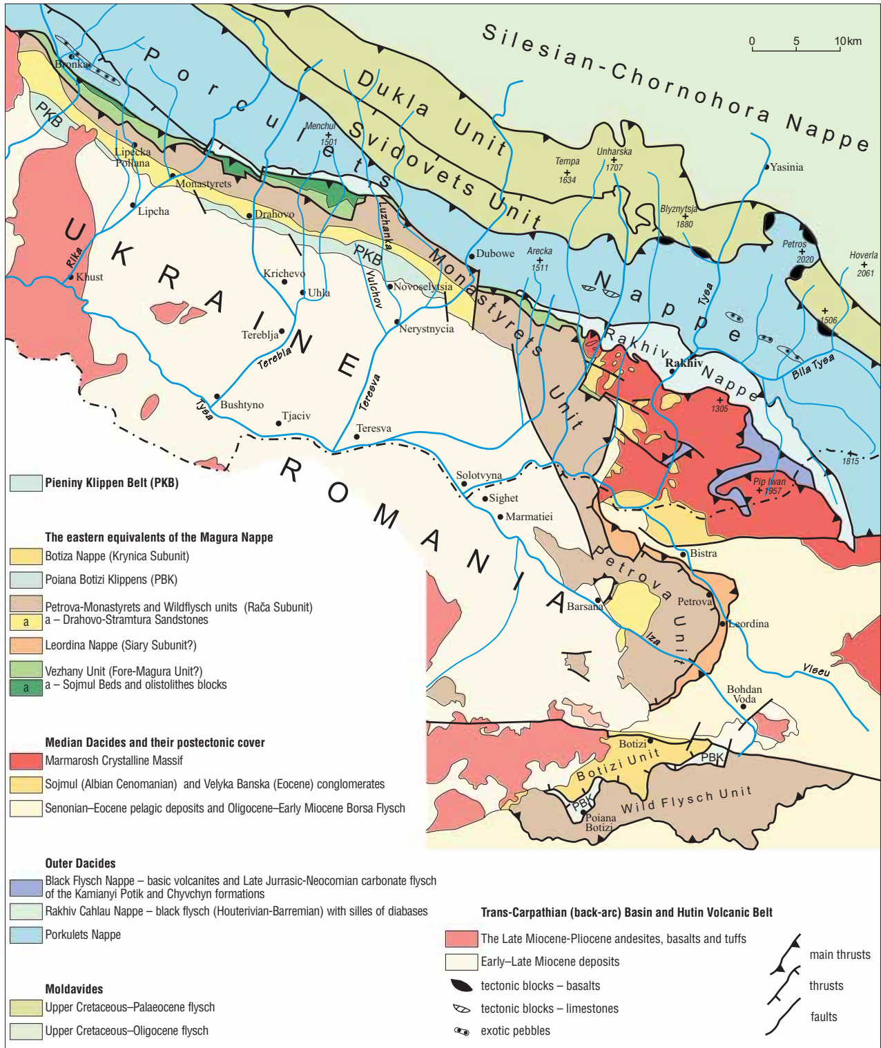
Fig. 7. Geological sketch-map of the SE part of the Ukrainian Carpathians and adjacent part of the Romanian Maramures — based on Shakin et al. (1976), Burov et al. (1986) and Aroldi (2001)
