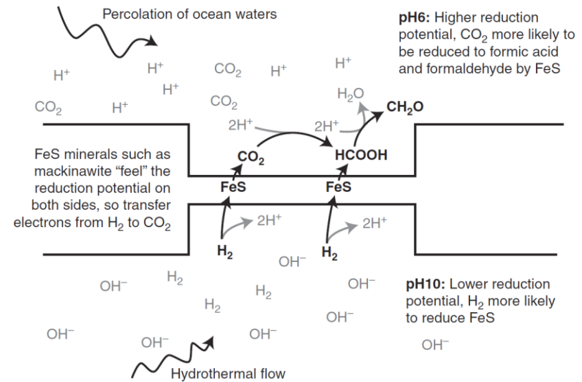
Figure 1. Proposed vectorial reduction of CO 2 by H 2 across a thin FeS barrier. The reduction potential ( E_h ) of the H + /H 2 couple is -590 mV at pH 10, whereas the E_h of the CO 2 /HCOOH couple at pH 6 is -370 mV, and the E_h of the HCOOH/CH 2 O is -520 mV. A semiconducting FeS barrier should "feel" the distinct reduction potentials in both compartments and transfer electrons from H 2 to CO 2 , to produce simple organics such as formaldehyde (CH 2 O).
