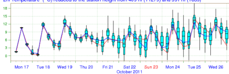
2m Temperature (°C) reduced to the station height from 409 m (T1279) and 391 m (T639)
