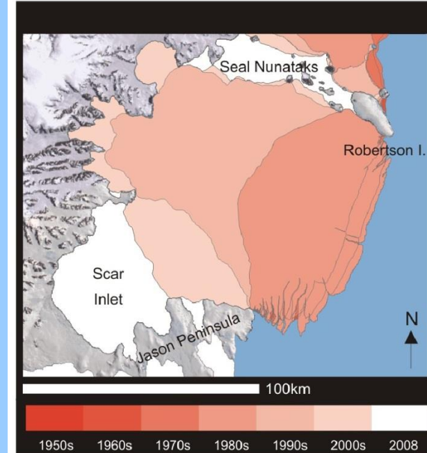
Larsen B Ice Shelf
