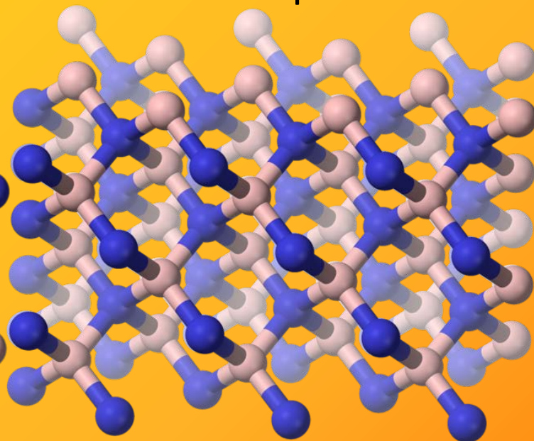
\beta - BN
