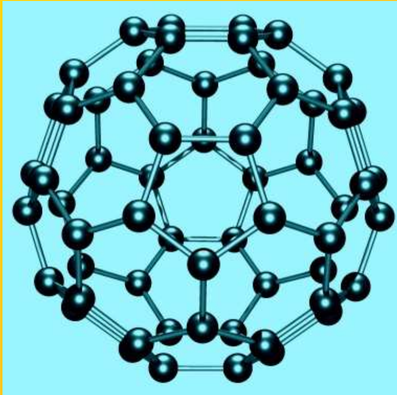
Fulleren C_{60}
