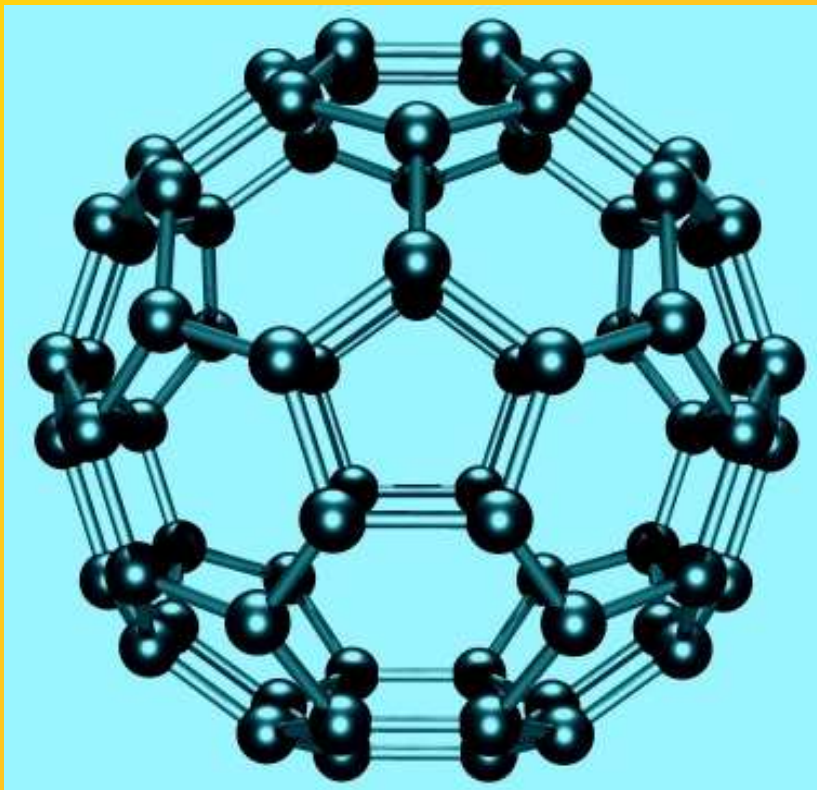
Fulleren \text{C}_{70}
