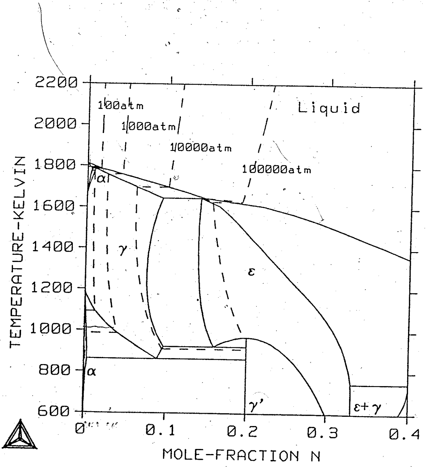
Fig.16. The calculated Fe-N phase diagram.
