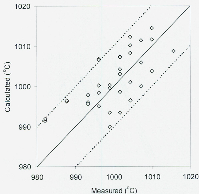
Fig. 27—A correlation of the thermodynamically calculated beta transus, i.e. , from the beta (bcc) phase to the alpha (hcp) phase using PANDAT and PanTitanium with actual measured values for Ti6Al4V. The experimental data were provided by D. Furrer, Ladish Co. (Cudahy, WI).
