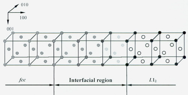
Fig. 39—A schematic supercell with a (100) IPB between an fcc (A1) phase and an L1_2 phase in a binary A-B. The black spheres represent A atoms such as Cu and Ni and the white spheres B atoms such as Au and Al. The gray color with differing intensities represents solution (A, B) with differing concentrations. The left side of this supercell represents the fcc (A1) phase and the right side the L1_2 phase. Only four lattice planes are shown but in reality there are many more than four.
