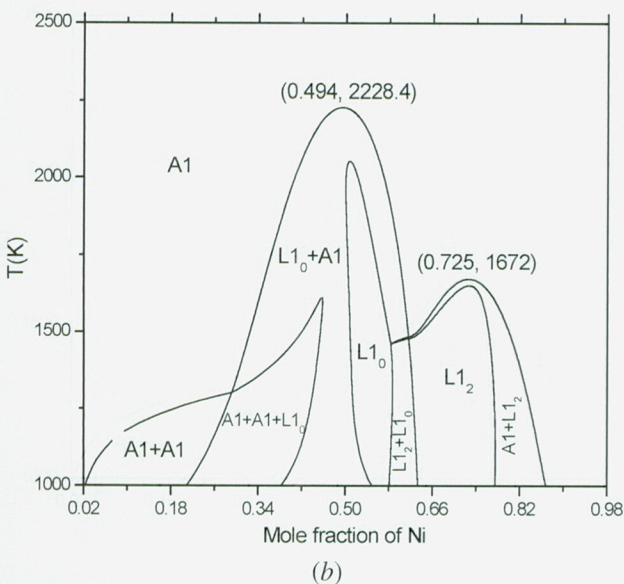
Fig. 31—CSA-calculated metastable fcc phase diagrams: (a) binary Ni-Al [106] and (b) an isopleth of Ni-Al-Cr with x_{Cr} = 0.02 . [108]
