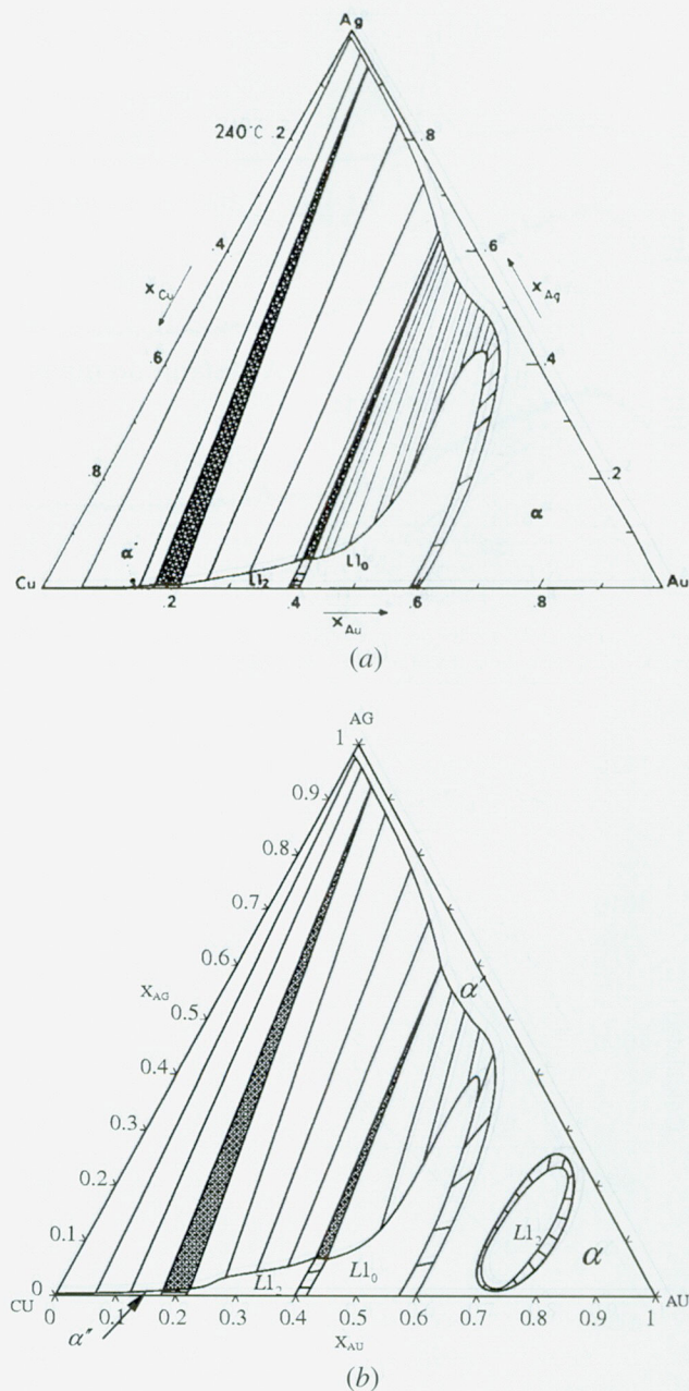
Fig. 28—Calculated coherent isotherms of Cu-Ag-Au at 240 °C: (a) CVM [111] and (b) CSA. [107]
