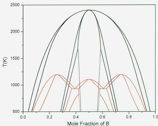
Fig. 37—Two ordering phase diagrams for the fcc phases calculated by the CEF and the modified CEF using the energy parameter and reciprocal parameters given in Figs. 35 and 36, respectively.
