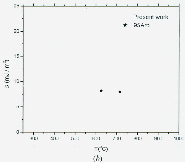
Fig. 43—(a) Comparisons of TP-CSA-calculated coherent IPB energies between fcc-(Al) and L_{12}\text{-Al}_3\text{Li} [122] with the TO-CVM values [123] and the experimental data. [125,126] (b) Comparisons of TP-CSA-calculated coherent IPB energies between \gamma and \gamma' in Ni-Al [122] with experimental data. [127,128]
