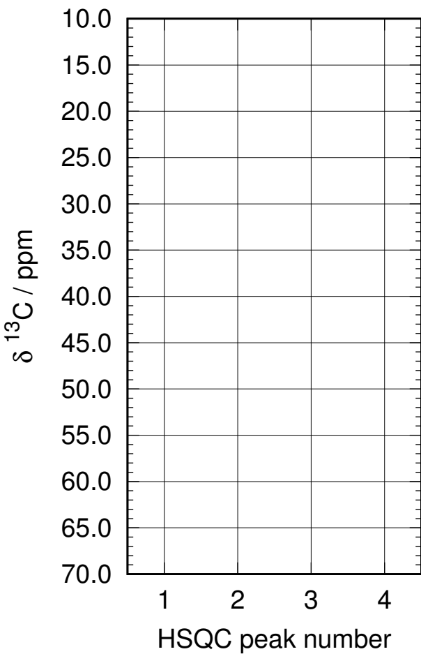
HNCACB Spectrum 7
