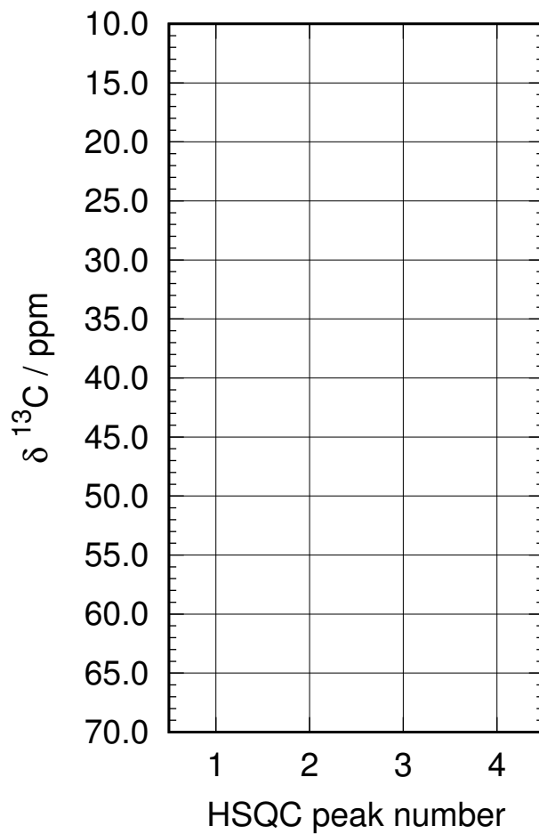
CBCA(CO)NH Spectrum 7
