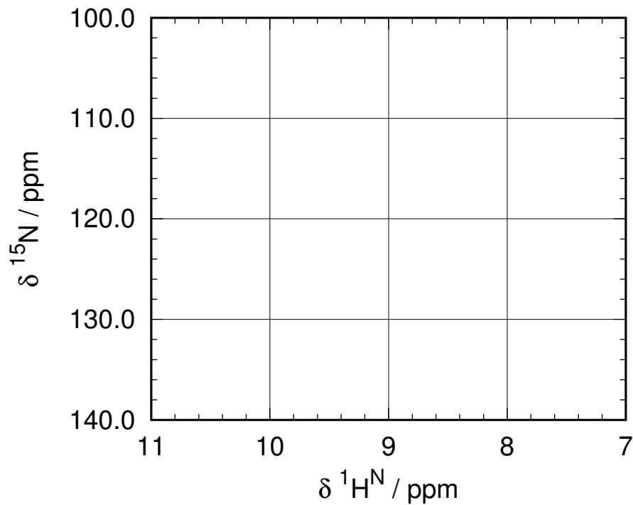
HSQC Spectrum
