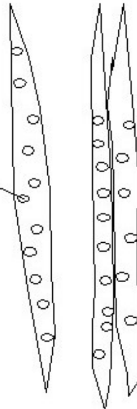
TRACHEIDS
