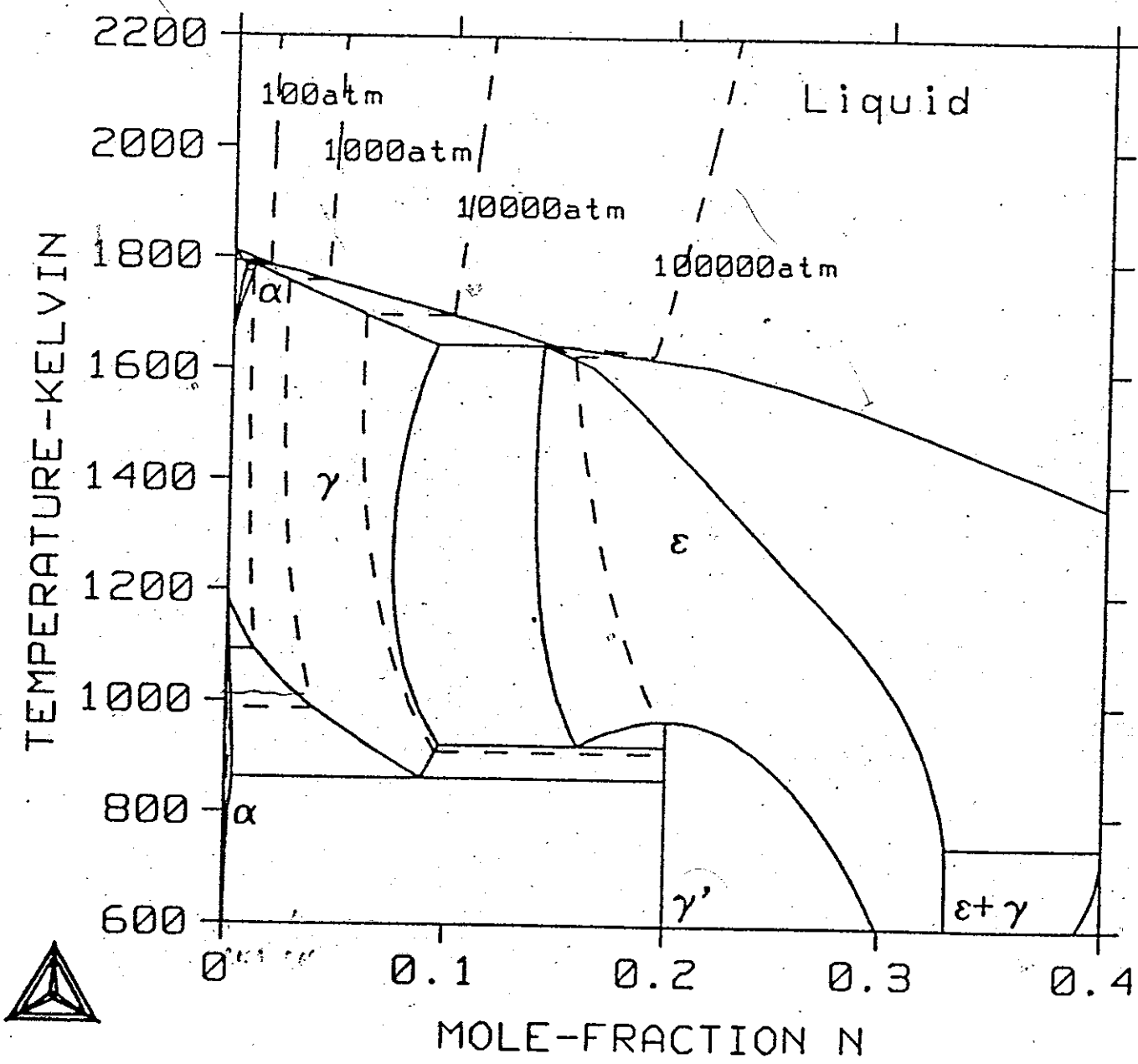
Fig.16. The calculated Fe-N phase diagram.
