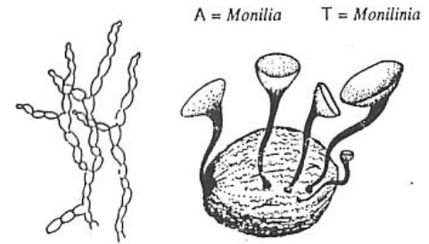
4.10 Leotialean holomorph.
