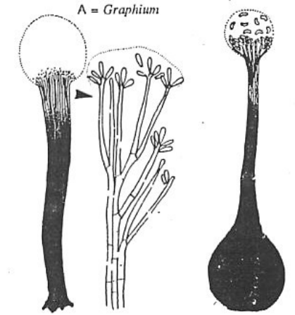
4.8 Ophiostomatalean holomorph.
