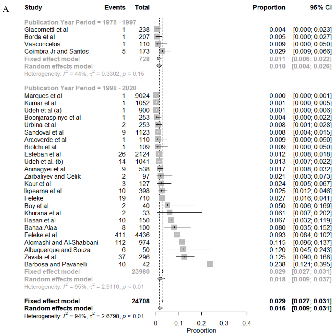
Fig. 2. Forest plot of the epidemiological studies retrieved on human balantidiasis analyzed according to the subgroups: (A) Year of publication, and (B) Continent of publication.
