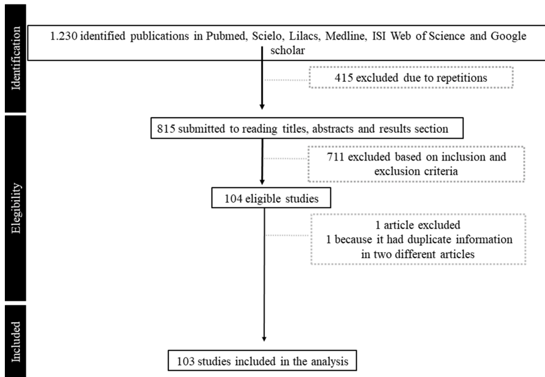
Fig. 1. Flowchart of the selection of articles on human balantidiasis analyzed in the systematic review and meta-analysis.
