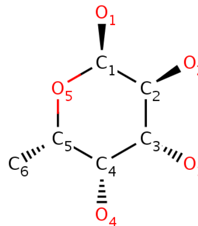
FUC, alpha -L-fucose
