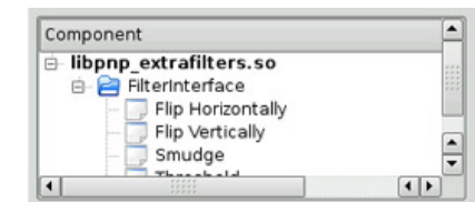
QTreeView
