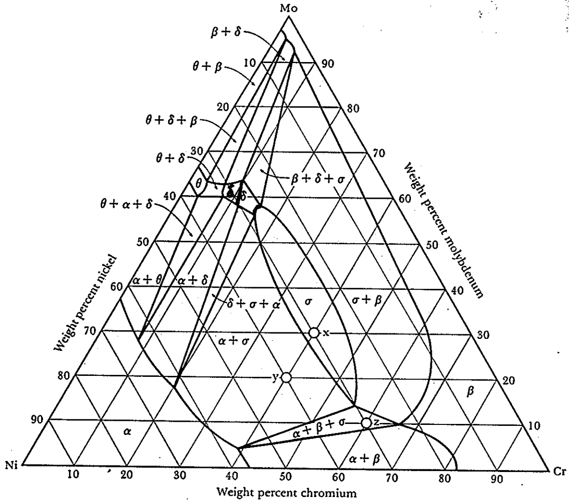
FIG. 10-26 An isothermal plot at 1250°C for the nickel-chromium-molybdenum ternary phase diagram.
