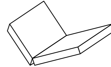
Buckle ( \kappa )
