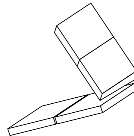
Tilt ( \tau )
