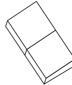
Inclination ( \eta )
