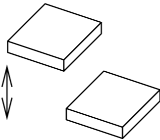
Stagger ( S_z )
