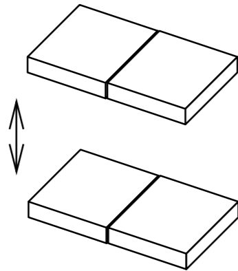
Stagger ( S_z )
